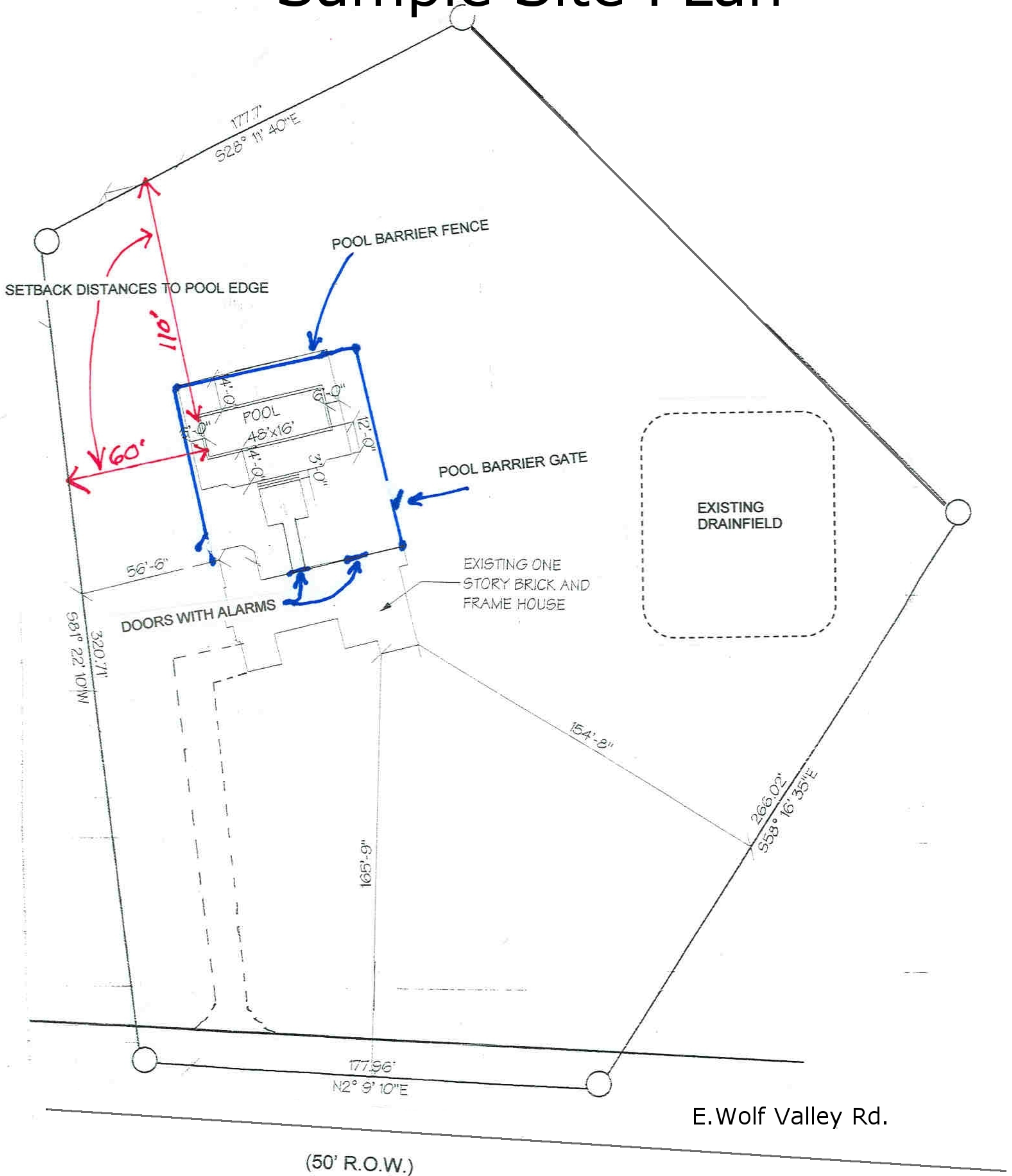
PLAT OF PROPERTY SHOWING PROPOSED POOL
